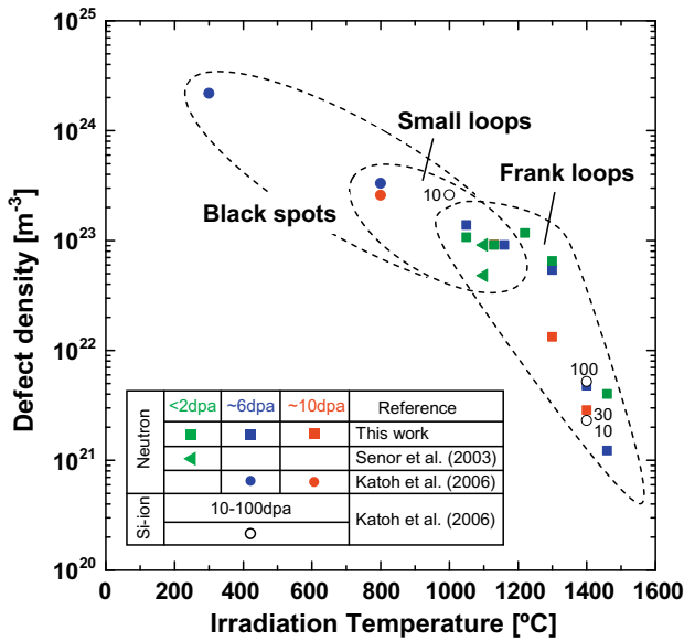
Fig. 5. Irradiation temperature dependence of defect number density in neutron-irradiated \beta -SiC. Displacement damage levels are indicated for the reported self-ion data.
