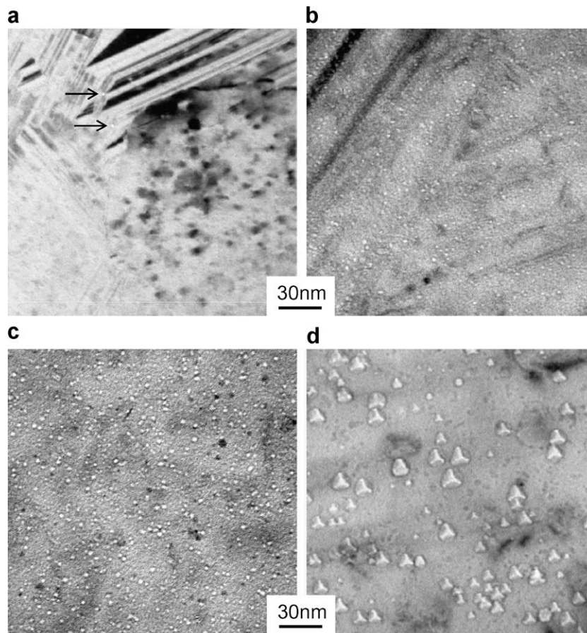
Fig. 1. Cavity microstructures in \beta -SiC irradiated at (a) 1050 °C, 4.9 dpa, (b) 1300 °C, 9.3 dpa, (c) 1400 °C, 9.4 dpa, and (d) 1460 °C, 5.6 dpa.
