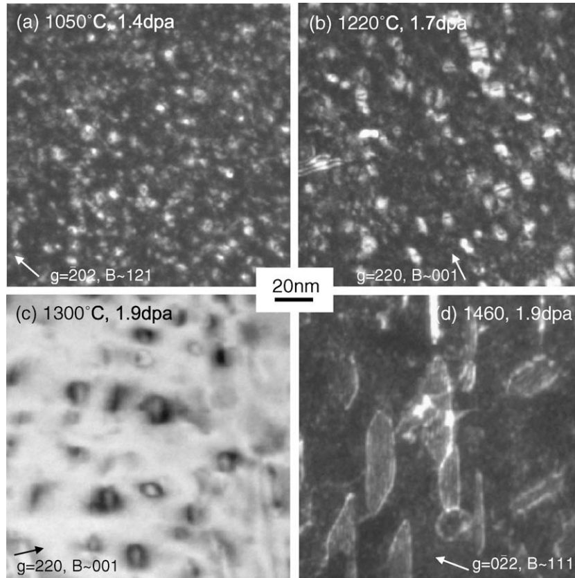
Fig. 4. Dislocation microstructures in \beta -SiC irradiated at (a) 1050 °C, 1.4 dpa, (b) 1220 °C, 1.7 dpa, (c) 1300 °C, 1.9 dpa, and (d) 1460 °C, 1.9 dpa. Beam direction and g vectors are indicated in each image.
