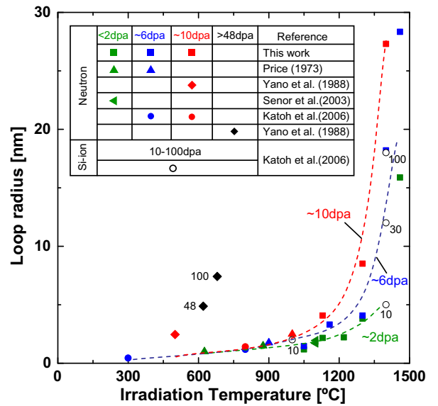
Fig. 6. Irradiation temperature dependence of defect size in neutron-irradiated \beta -SiC. Displacement damage levels are indicated for the reported self-ion data and some neutron data obtained at much higher fluencies compared to this work.
