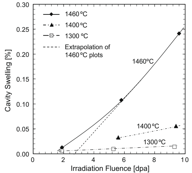
Fig. 3. Irradiation fluence dependence of cavity swelling in neutron-irradiated \beta -SiC at three temperatures.
