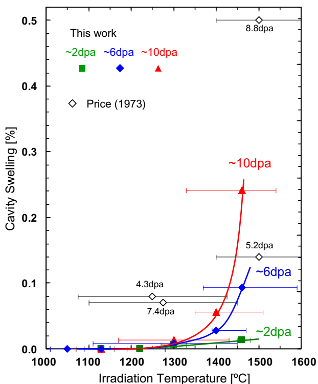
Fig. 2. Irradiation temperature dependence of cavity swelling in neutron-irradiated \beta -SiC.
